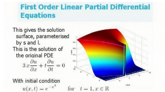
Figure 1. First Order Partial Differential Equations [16]
