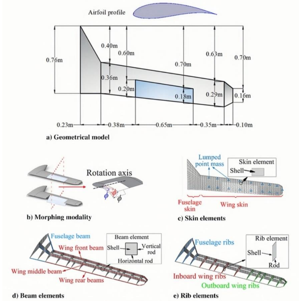
Figure 3. Structural design of the morphing wing [23]
